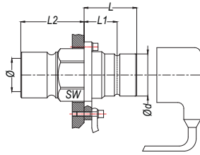
with female thread
