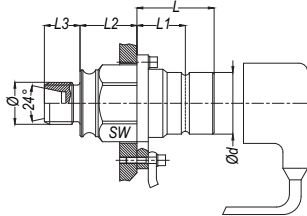
with male thread hydraulic pipes with 24° cone
